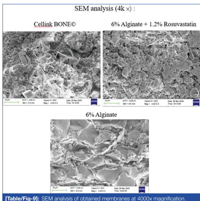
[Table/Fig-9]: SEM analysis of obtained membranes at 4000x magnification.
